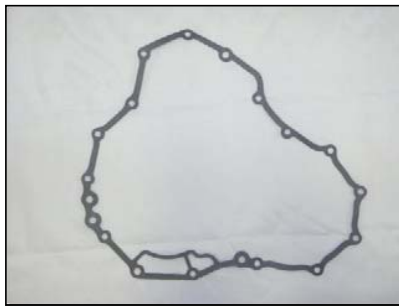
48797 K48900F CASE ID: B7VA, B7YA, B7TA, B7XA 1999 3.2TL, 2000-02 ACCORD (V6), 1999-01 ODYSSEY OEM #21812-P7Z-000
