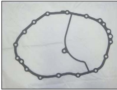
98536 K98900F CASE ID: SPSA, SMLA, STYA, SBLA 2010-12 CIVIC HYBRID, 2011-12 CR-Z, 2010-12 INSIGHT OEM #21813-RBL-000
