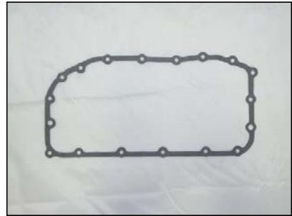
98814 K98900J CASE ID: SZCA (CVT) 2003-04 CIVIC HYBRID OEM #21814-PZC-000
