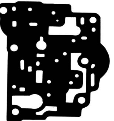
Part: 79184 OE#: N/A Trans: TF-80SC (AF40) TF81SC (AF21) Appl: Aux V/B separator plate to cover Kit#: K79900G
