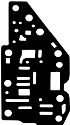
Part: 79960 OE#: N/A Trans: 09G Appl: Sml Aux V/B to plate Kit#: K79900H
