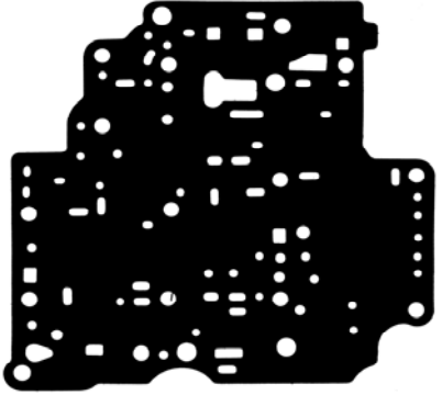
Part: 79906 OE#: 90348906 Trans: AW50-40LE (AF-14, AF-20) Appl: Aux V/B Upper Kit#: K79900, K79900A, K79900B
