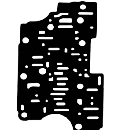
Part: 79951 OE#: N/A Trans: 09G Appl: Lg Aux V/B to plate Kit#: K79900H
