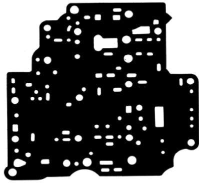
Part: 79084 OE#: 90543084 Trans: AW50-42LE (AF-22) Appl: Aux V/B Upper Kit#: K79900B, K79900C
