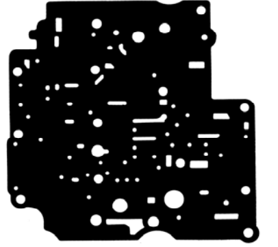
Part: 79067 OE#: N/A Trans: AW55-50SN/AW55-40 (AF-23, 33), RE5F22A (AW55-51SN) Appl: Aux V/B #2 (Exc Volvo, Renault) Kit#: K79900N
