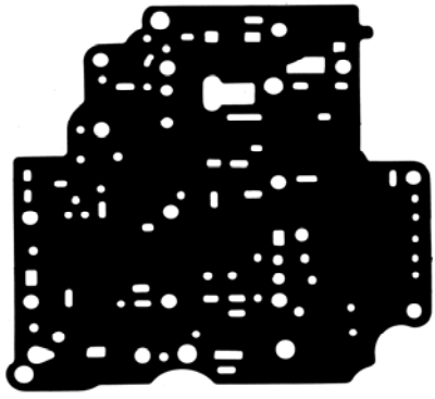
Part: 79050 OE#: N/A Trans: AW50-40LE (AF-14, 21) Appl: Aux V/B Upper (Saab only) Kit#: K79900C
