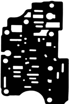
Part: 79950 OE#: N/A Trans: 09G Appl: Lg Aux V/B plate to cover Kit#: K79900H
