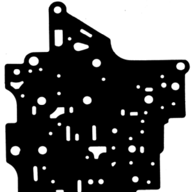
Part: 79066 OE#: N/A Trans: AW55-50SN/AW55-40 (AF-23, 33), RE5F22A (AW55-51SN) Appl: Aux V/B #1 (Exc Volvo, Renault) Kit#: K79900N
