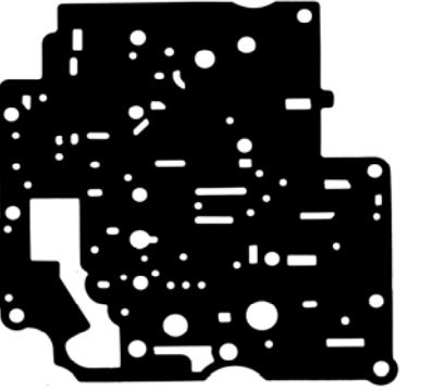
Part: 79041 OE#: N/A Trans: AW55-50SN/AW55-40 (AF-23, 33), RE5F22A (AW55-51SN) Appl: Aux V/B #2 (Volvo, Renault) Kit#: K79900N
