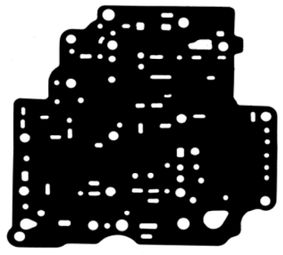
Part: 79905 OE#: 90348905 Trans: AW50-40LE (AF-14, AF-20) Appl: Aux V/B Lower Kit#: K79900, K79900A, K79900B
