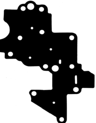
Part: 79015 OE#: N/A Trans: AW60-41SN (AF-17) Appl: V/B Pre main Kit#: K79900E
