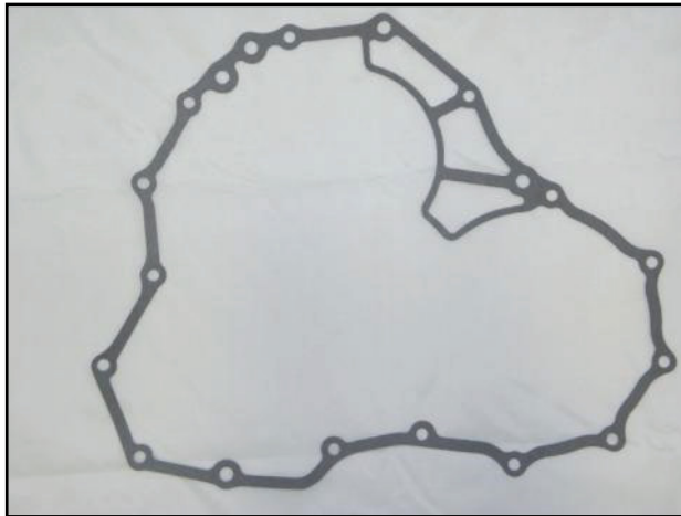
48313 K48900L CASE ID: M7WA, B7WA, BGFA, MGFA, MGHA, BYBA, BDGA, BGHA, BAYA, MAYA 2000-06 3.2TL, 2001-02 MDX, 2001-03 3.2CL, 2002 ODYSSEY, 2006-07 ACCORD (V6) OEM #21812-P7W-000, 21812-PGH-010, 21812-RDG-000
