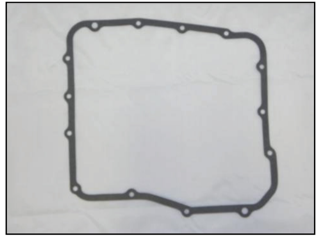
48218 K48900Y CASE ID: MPYA, M5HA, M5DA, 1995 LEGEND AFTER 5025383, 1995-98 3.2TL, 1996-01 3.5RL OEM #21813-P5H-000
