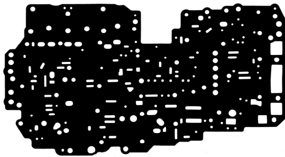
Part # 88204 A340E (Volvo Bonded) Valve Body Lower OE# N/A Kit # K88900L
