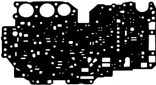
Part # 88906 A340E/F, A343F Valve Body Upper OE# 35433-60040 Kit # K88900DL
