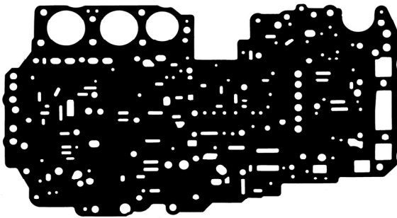
Part # 88203 A340E (Volvo Bonded) Valve Body Upper OE# N/A Kit # K88900L
