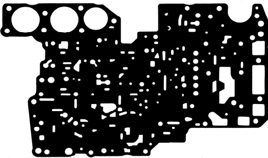
Part # 88904F A340/E Valve Body Upper OE# 35433-30063 Kit # K88900C, K88900D
