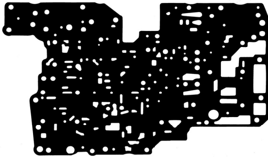
Part # 88903F A340/E Valve Body Lower OE# 35434-30072 Kit # K88900D
