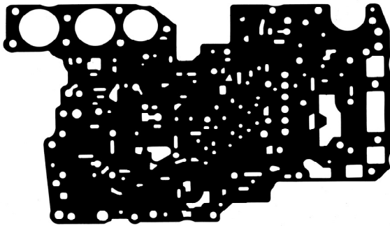
Part # 88904C AW4, A340E/F/H, A343F Valve Body Upper OE# 35433-30064 Kit # K88900C/D/DL/J/K/L/M/P
