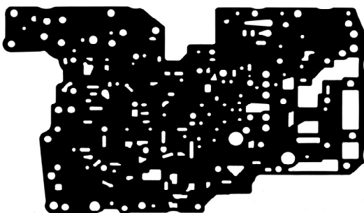
Part # 88903D A340 Valve Body Lower (Isuzu) OE# 8-97019-529-0 Kit # K88900D
