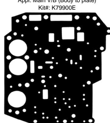
Part: 79580 OE#: N/A Trans:SR410-2, SR412-2 Appl: V/B Upper Kit#: K79900F
