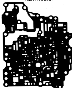
Part: 79193 OE#: N/A Trans: TF-80SC (AF40) Appl: Main V/B (Plate to pre-main V/B) Kit#: K79900G
