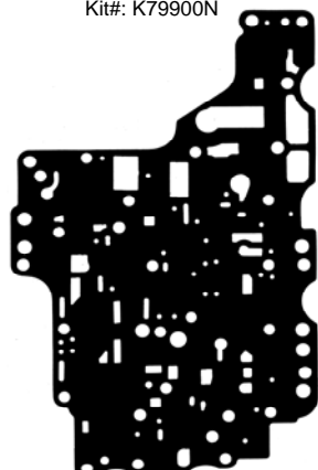
Part: 79010 OE#: N/A Trans: AW60-40LE/42LE (AF-13) Appl: Main V/B (Plate to cover) Kit#: K79900E
