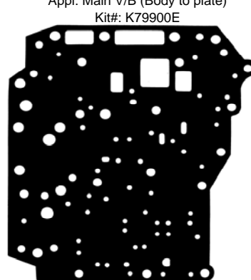
Part: 79481 OE#: N/A Trans:SR410-2, SR412-2 Appl: V/B Lower Kit#: K79900F
