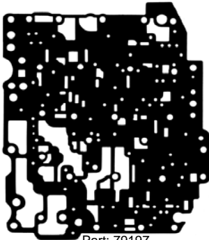
Part: 79197 OE#: N/A Trans: TF-81SC (AF21) Appl: Main V/B (V/B cover separator plate to main V/B) Kit#: K79900G
