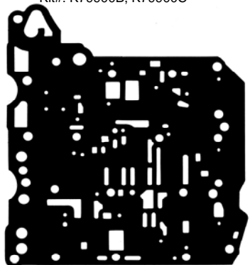
Part: 79756 OE#: N/A Trans: AW55-50SN/AW55-40 (AF-23, 33), RE5F22A(AW55-51SN) Appl: Main V/B Upper Kit#: K79900N
