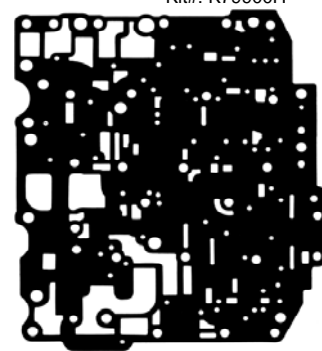
Part: 79195 OE#: N/A Trans: TF-81SC (AF21) Appl: V/B cover (V/B cover to cover separator plate) Kit#: K79900G
