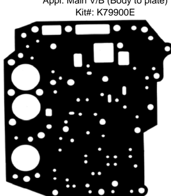
Part: 79480 OE#: N/A Trans:SR410-2, SR412-2 Appl: V/B Upper Kit#: K79900F
