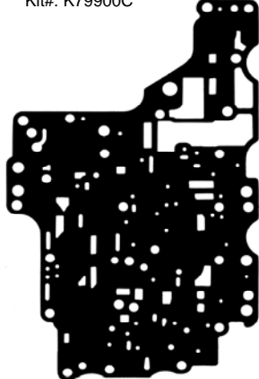
Part: 79011 OE#: N/A Trans: AW60-40LE/42LE (AF-13) Appl: Main V/B (Body to plate) Kit#: K79900E
